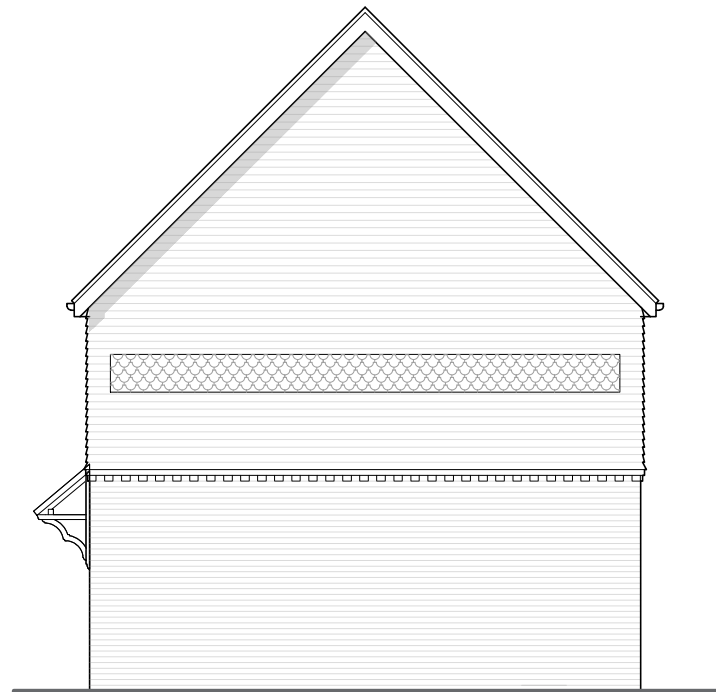
Elevation D
