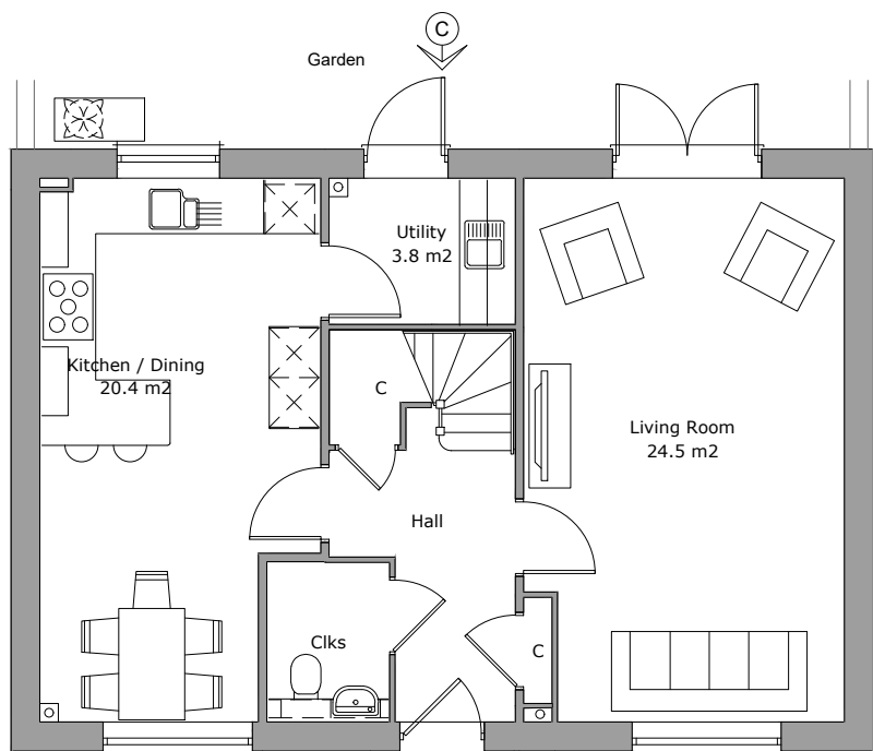
Ground Floor Plan Area 64.3m²
