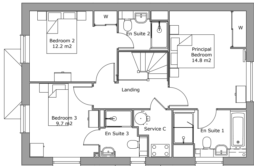
First Floor Plan Area 64.3m²
