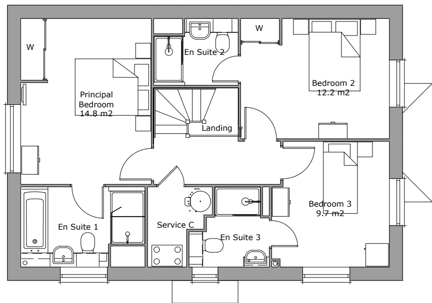
First Floor Plan Area 64.3m²
