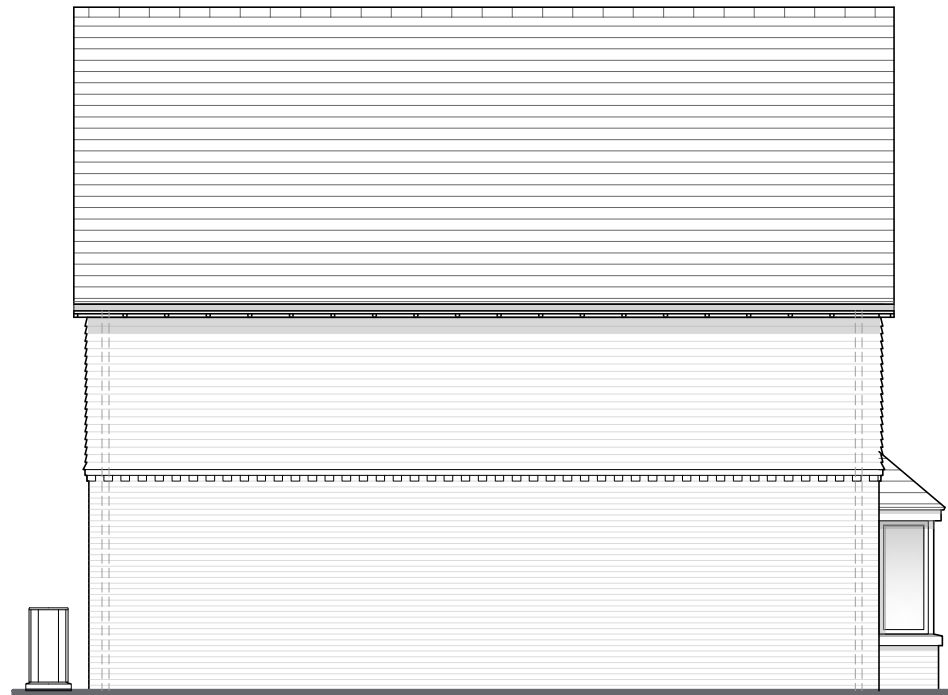
Elevation C
