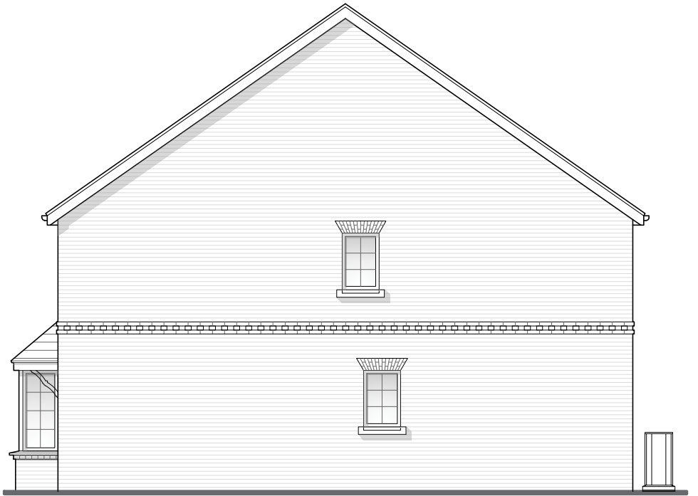
Elevation D
