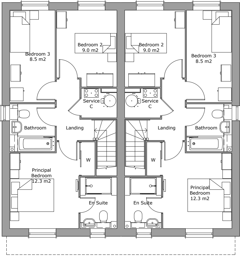
First Floor Plan Area 49.0m²
