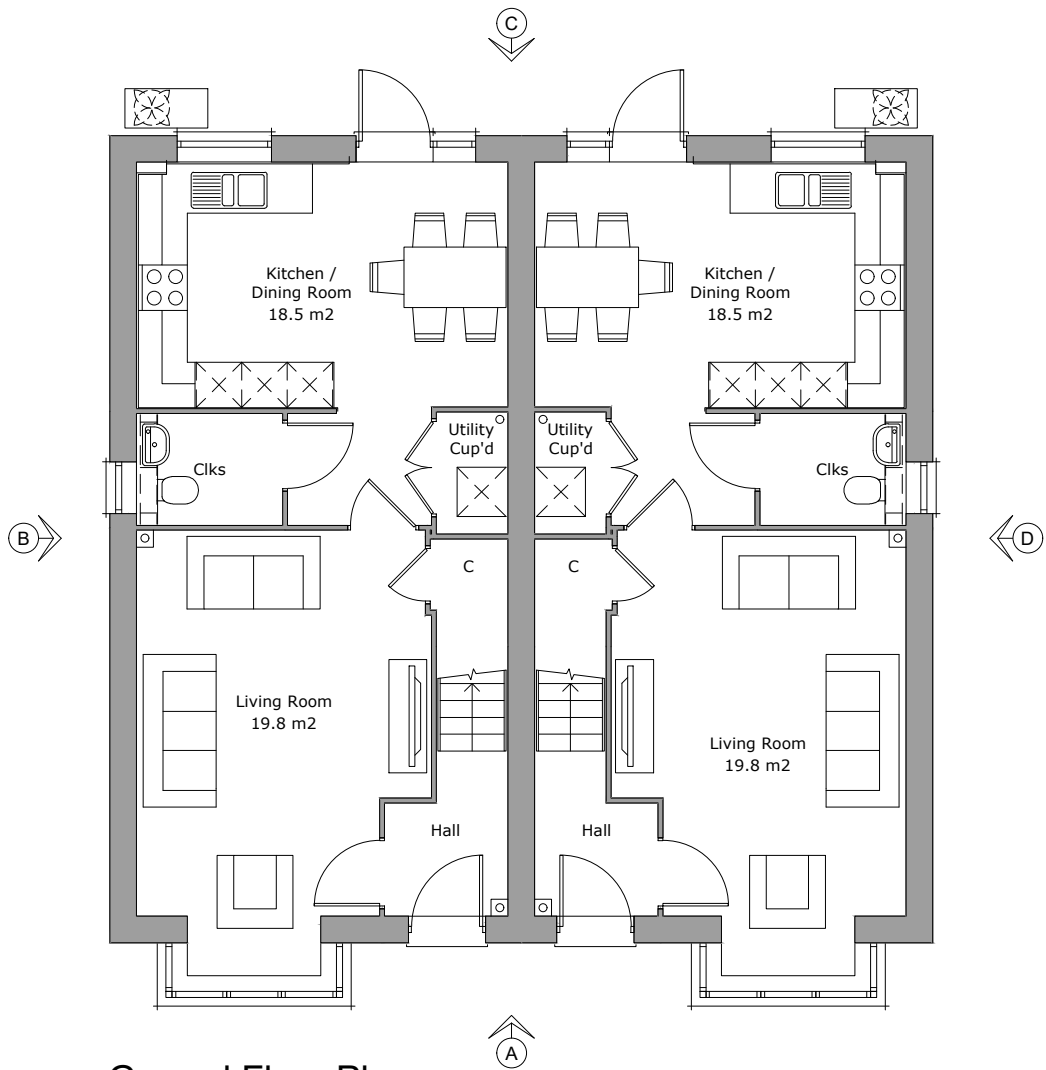
Ground Floor Plan Area 50.4m²
