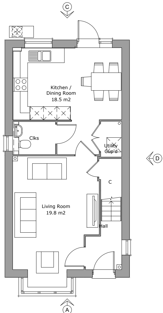
Ground Floor Plan Area 50.4m²
