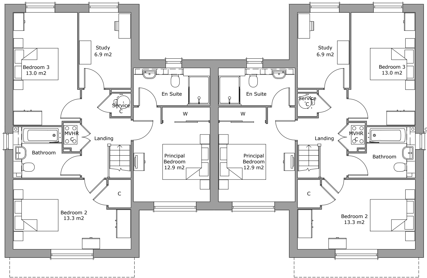
First Floor Plan Area 70.0m²
