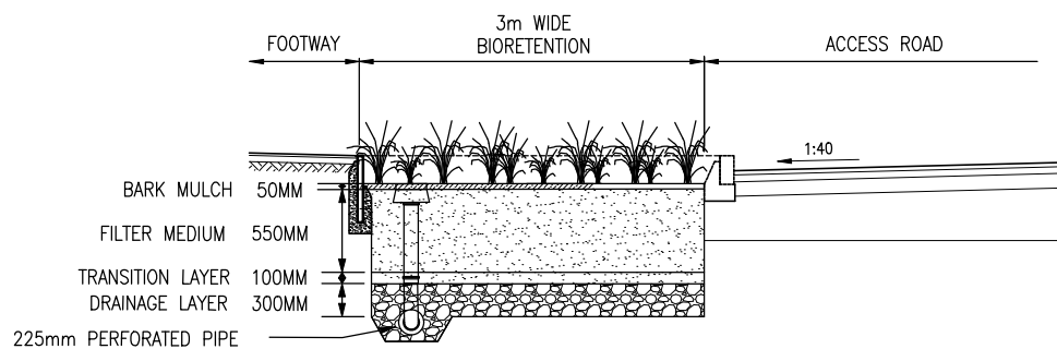
BIORETENTION DETAIL
