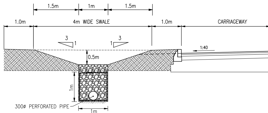
DRY SWALE DETAIL
