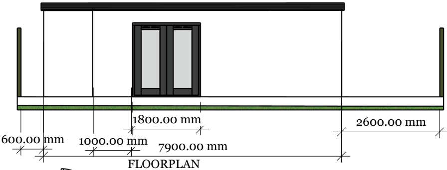
REAR ELEVATION
