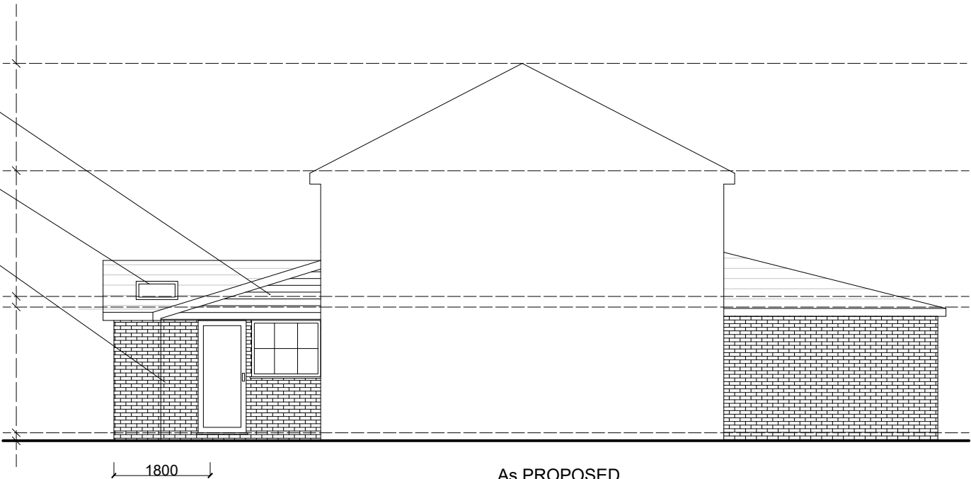
As PROPOSED
