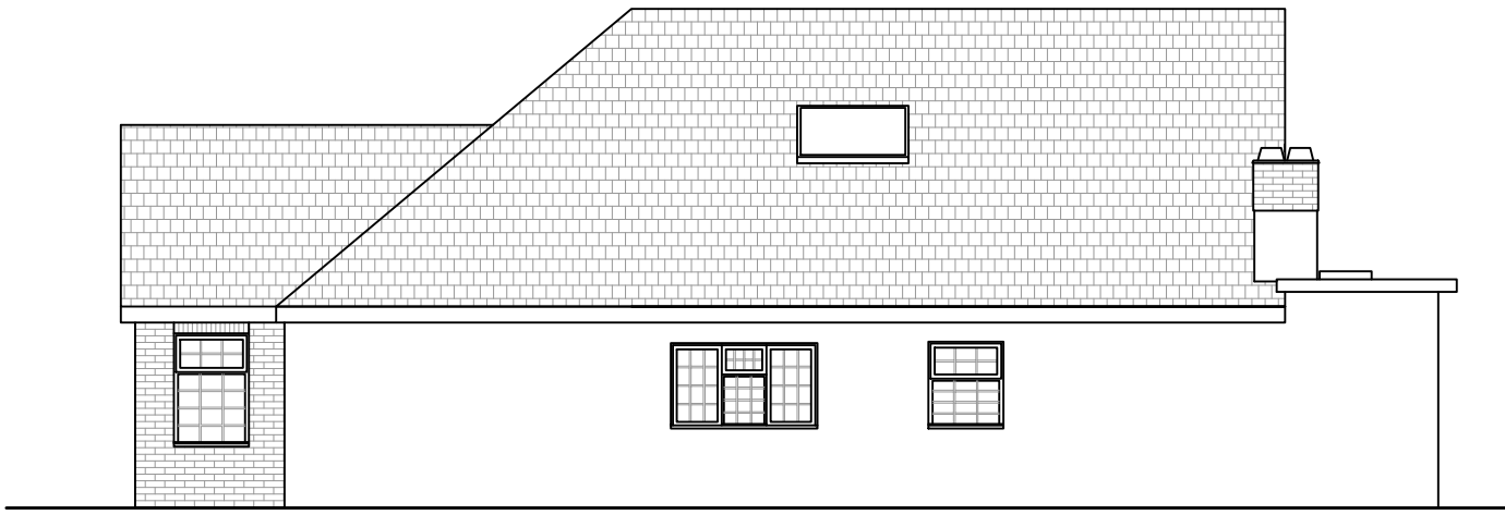
EXISTING RIGHT SIDE ELEVATION
