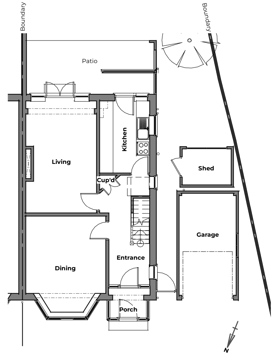
Existing Ground Level Plan General Arrangement | Scale 1:100
