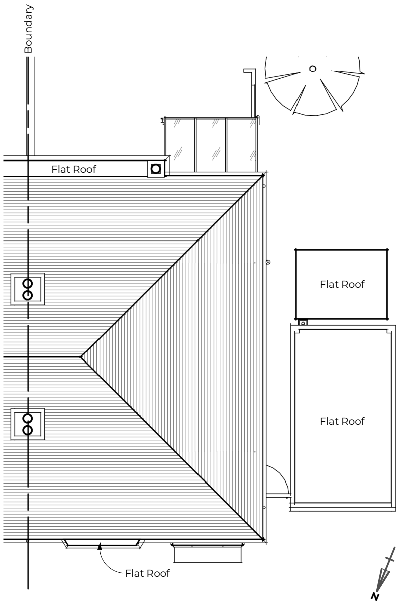
Existing Roof Level Plan General Arrangement | Scale 1:100
