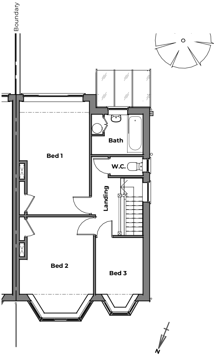
Existing First Level Plan General Arrangement | Scale 1:100
