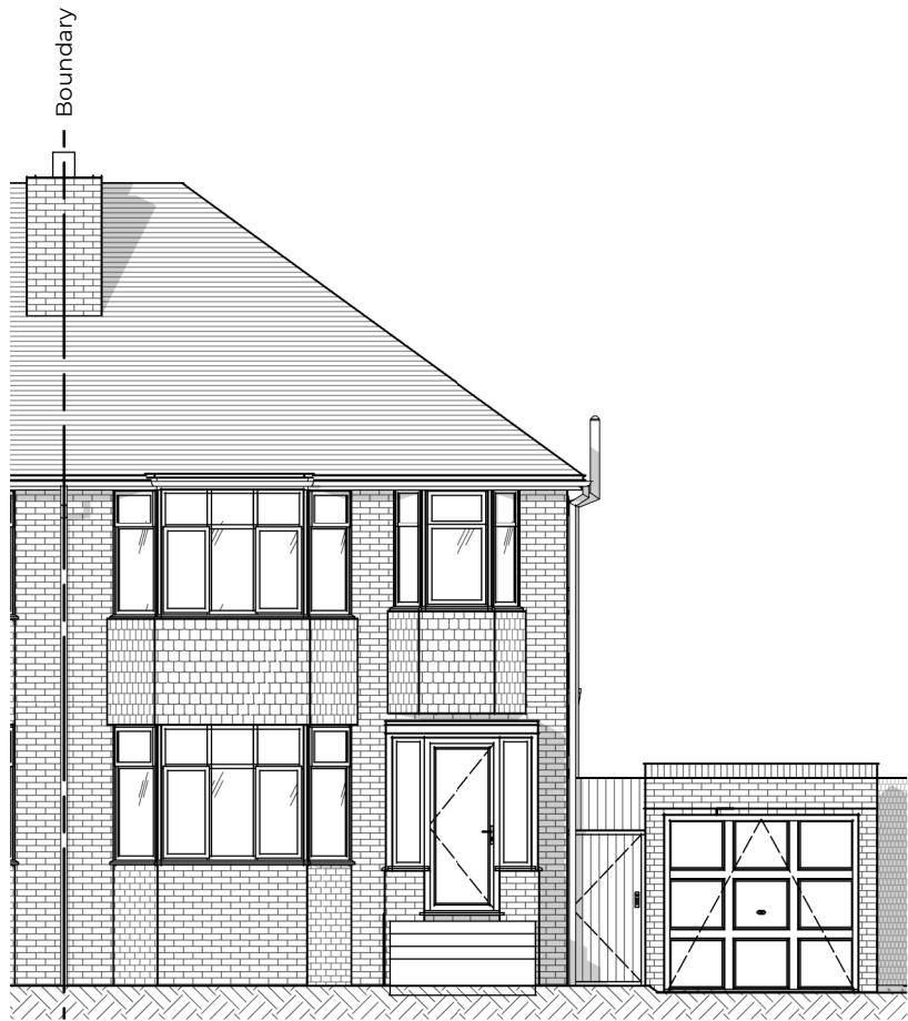
Existing Elevation - North
