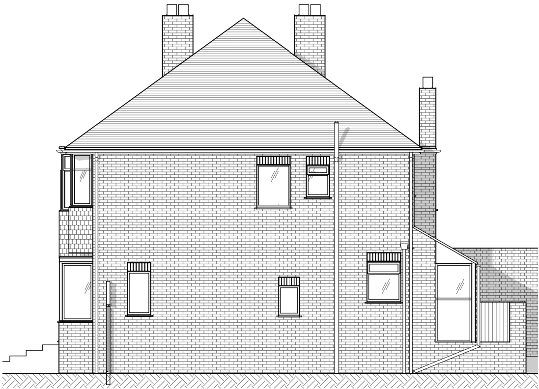
Existing Elevation - West
