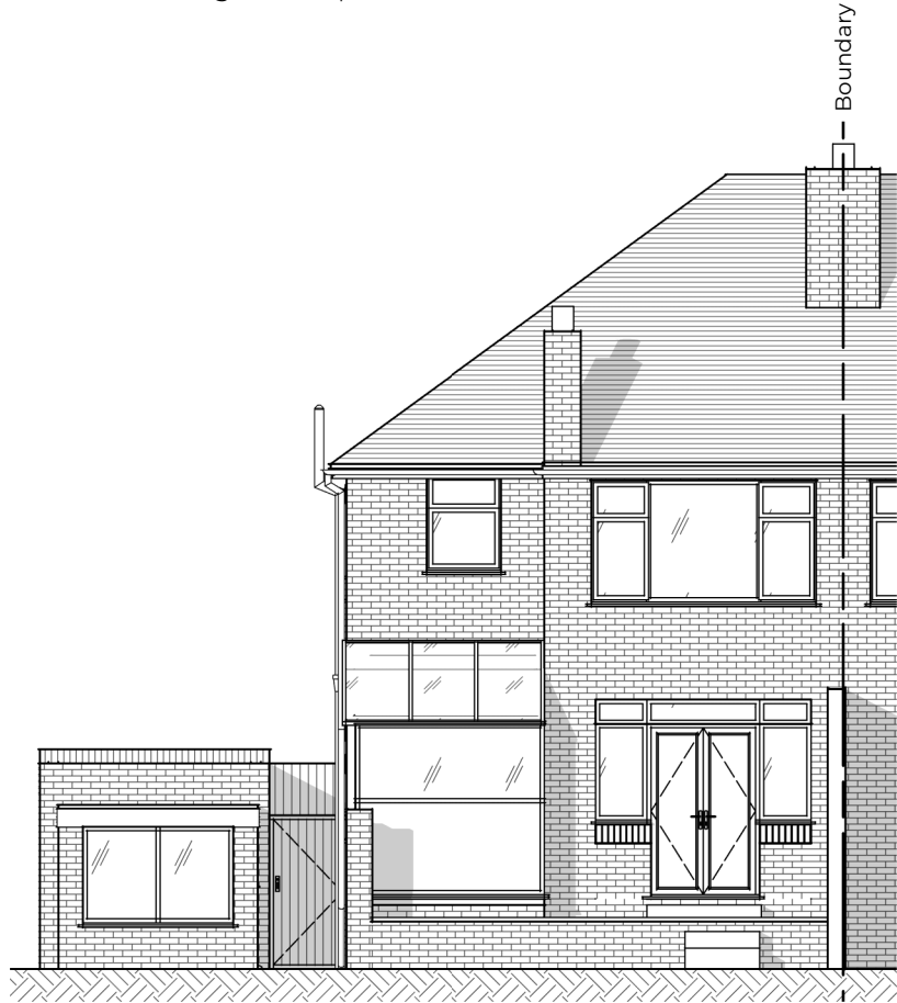
Existing Elevation - South
