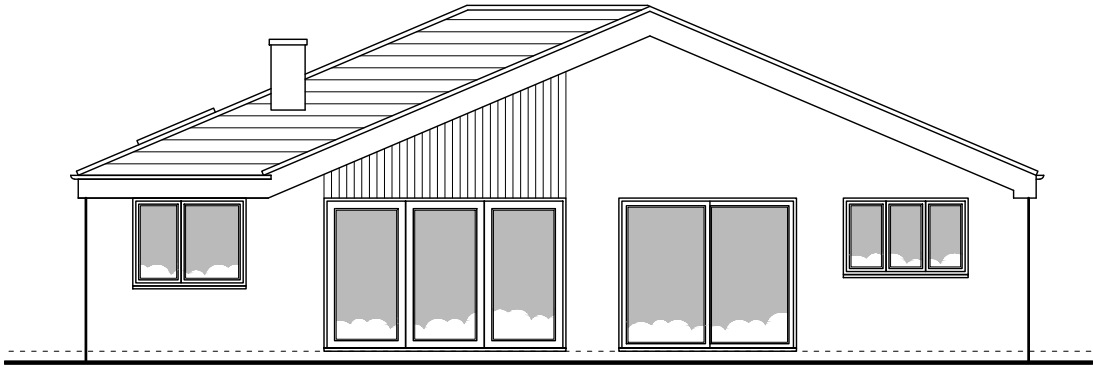
REAR ELEVATION 1:100
