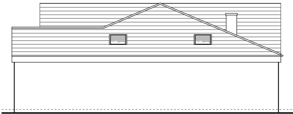
SIDE ELEVATION 1:100
