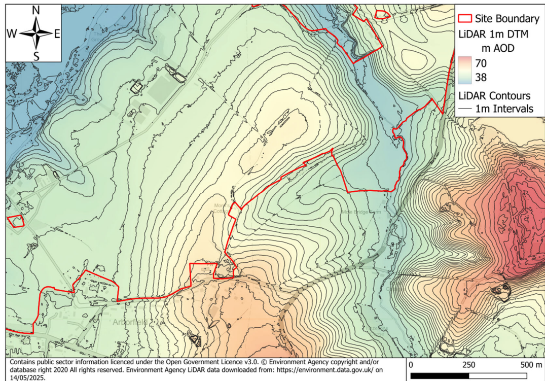
Figure 2C: Site Topography
