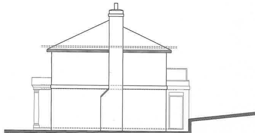
1:100 Proposed Rh side Elevation
