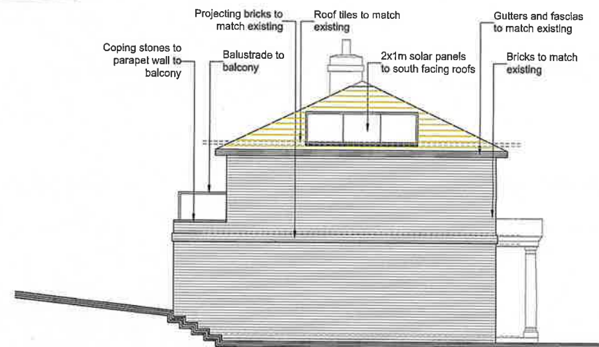
1:100 Proposed Lh side Elevation
