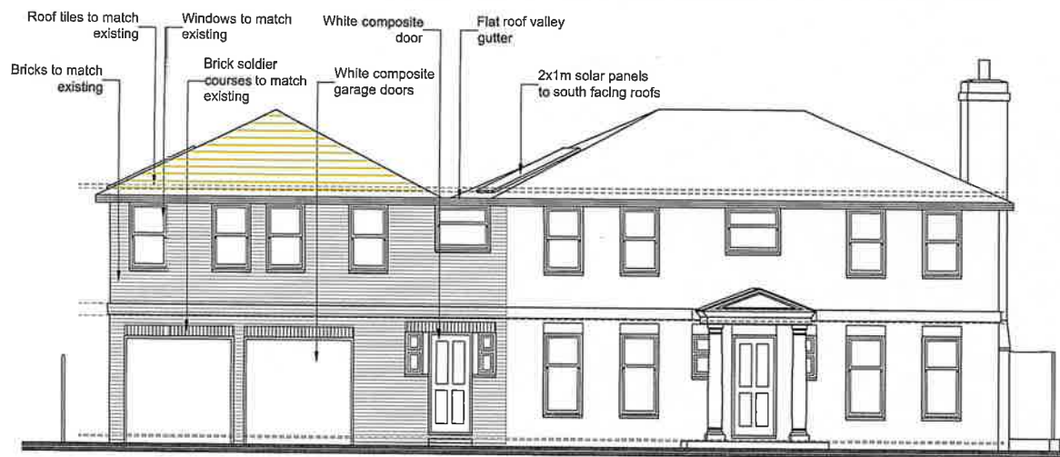
1:100 Proposed Front Elevation
