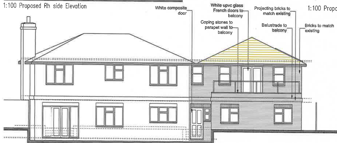
1:100 Proposed Rear Elevation
