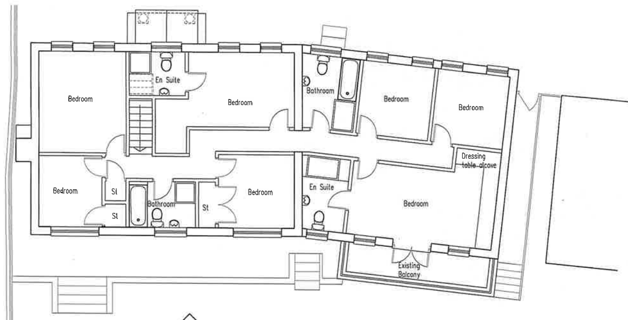
1:100 Proposed First floor plan
