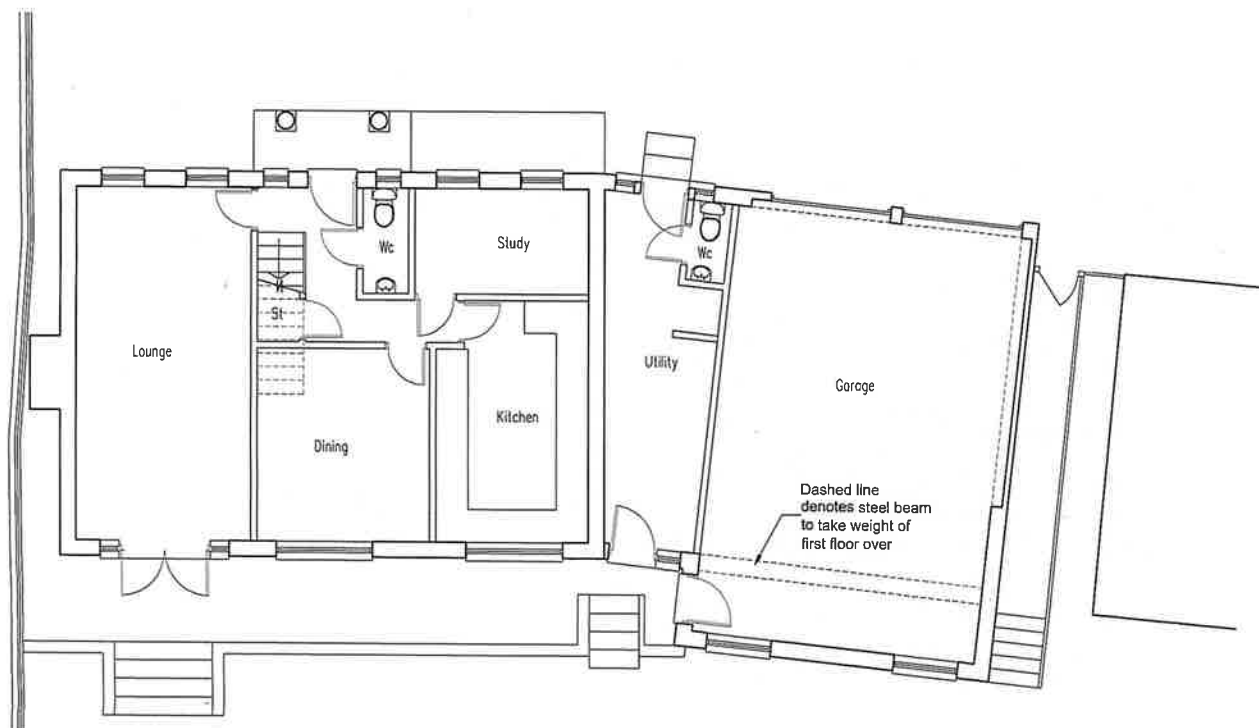
1:100 Proposed Ground floor plan
