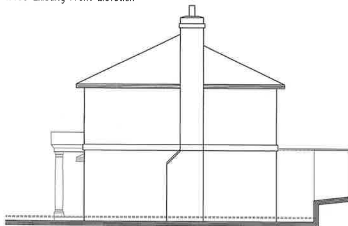
1:100 Existing Lh side Elevation
