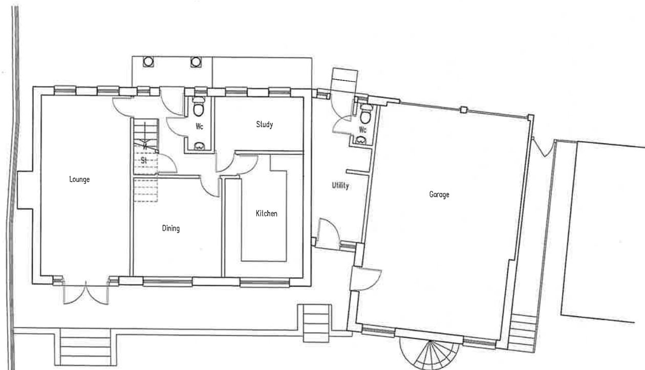
1:100 Existing Ground floor plan
