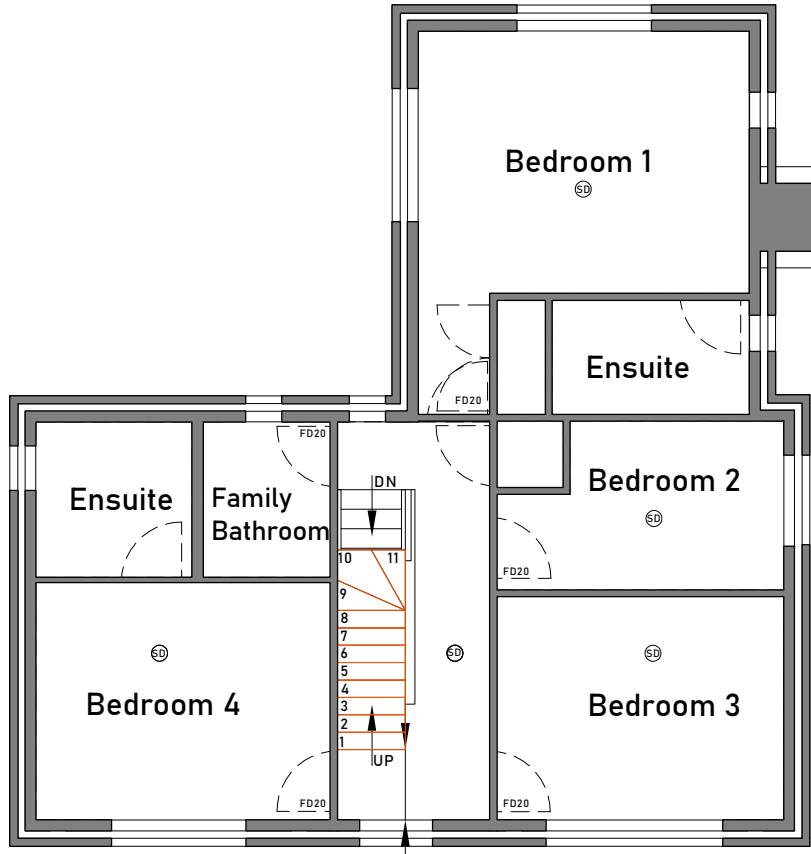
Proposed First Floor Plan (1:100 @ A3)
