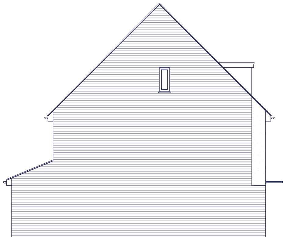
SIDE ELEVATION
