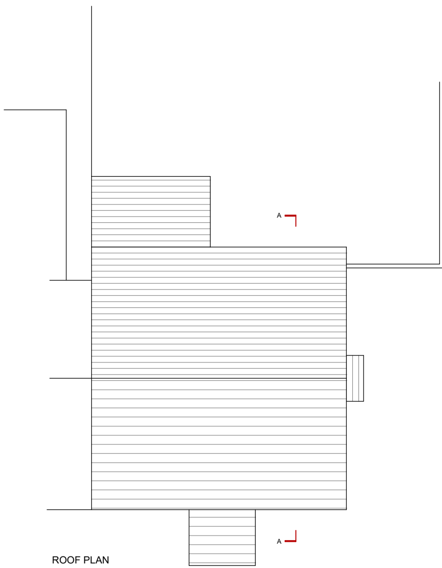
ROOF PLAN
