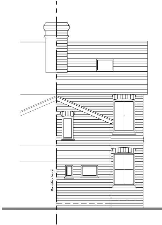
Rear Elevation
