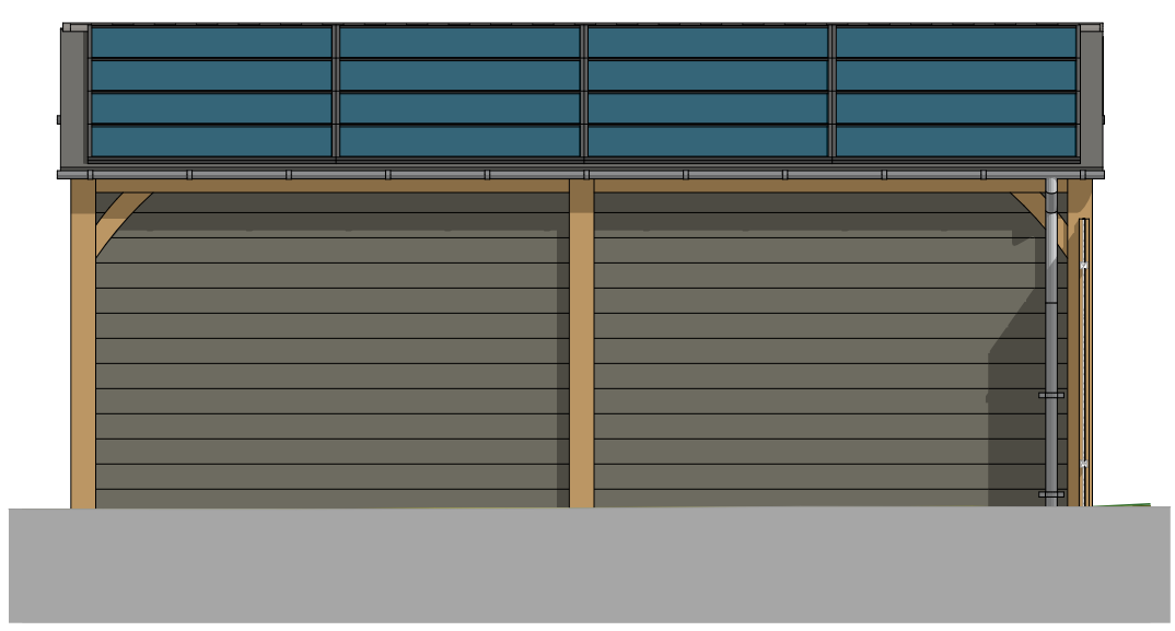
Approved Back Elevation 1:50
