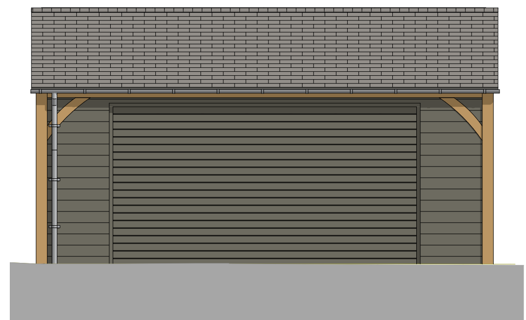
Proposed Front Elevation 1:50
