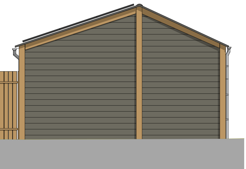
Proposed East Elevation 1:50
