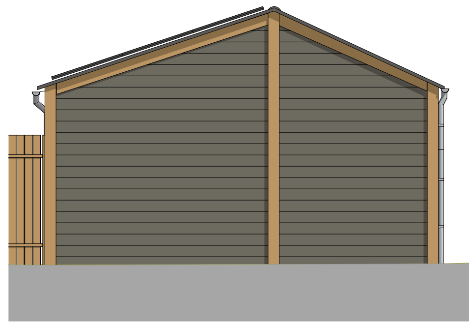
Garage East Elevation 1:50
