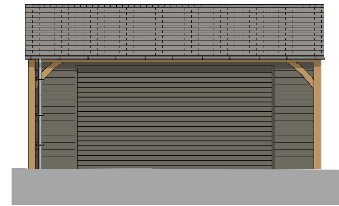
Garage Front Elevation 1:50
