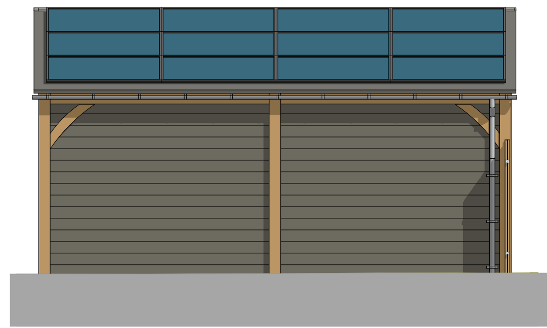
Garage Back Elevation 1:50
