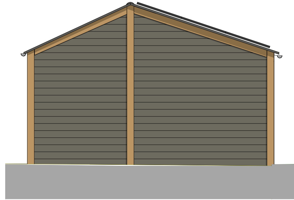
Garage West Elevation 1:50
