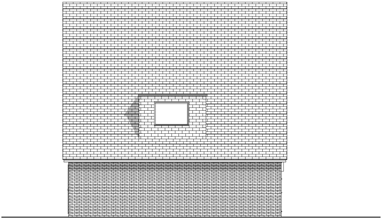
E-04 Existing Side left Elevation 1:100
