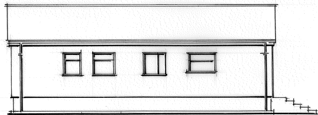
rear elevation west
