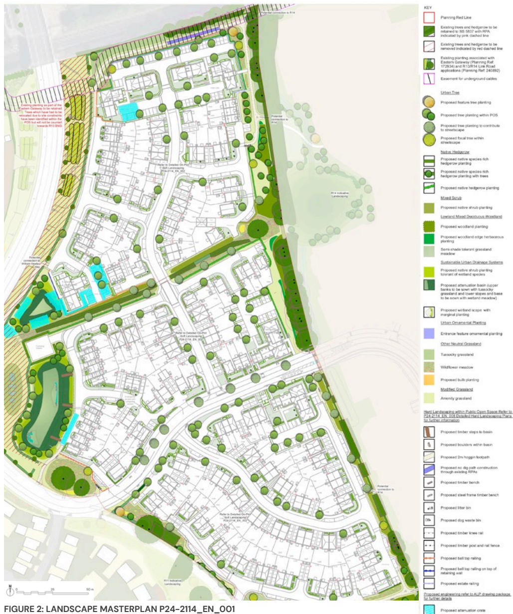
FIGURE 2: LANDSCAPE MASTERPLAN P24-2114_EN_001
