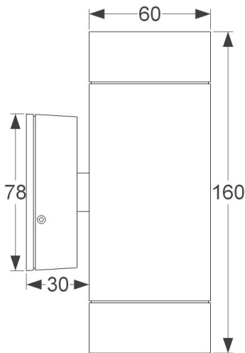
WALL2LBK GU10 Wall Mounted Fitting
