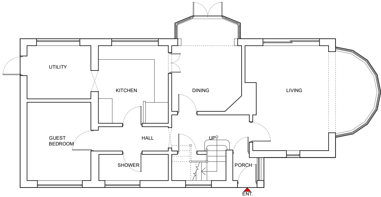
EXISTING GROUND FLOOR PLAN (GIA = 81.5m 2 )
