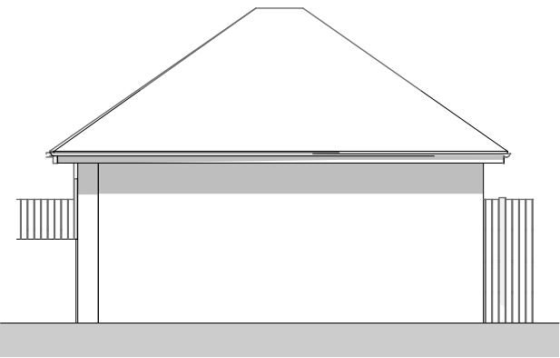
1:100 Right Side Garage Elevation
