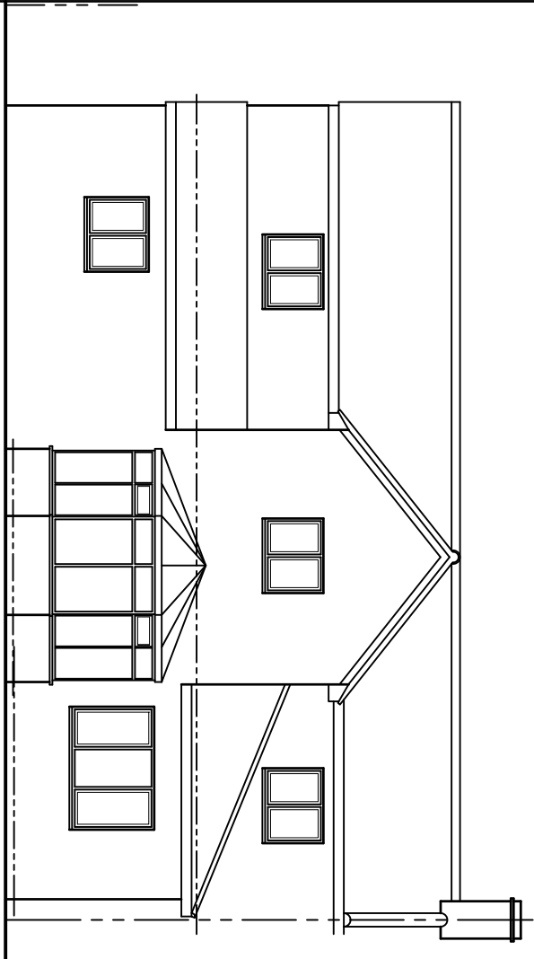
REAR ELEVATION
