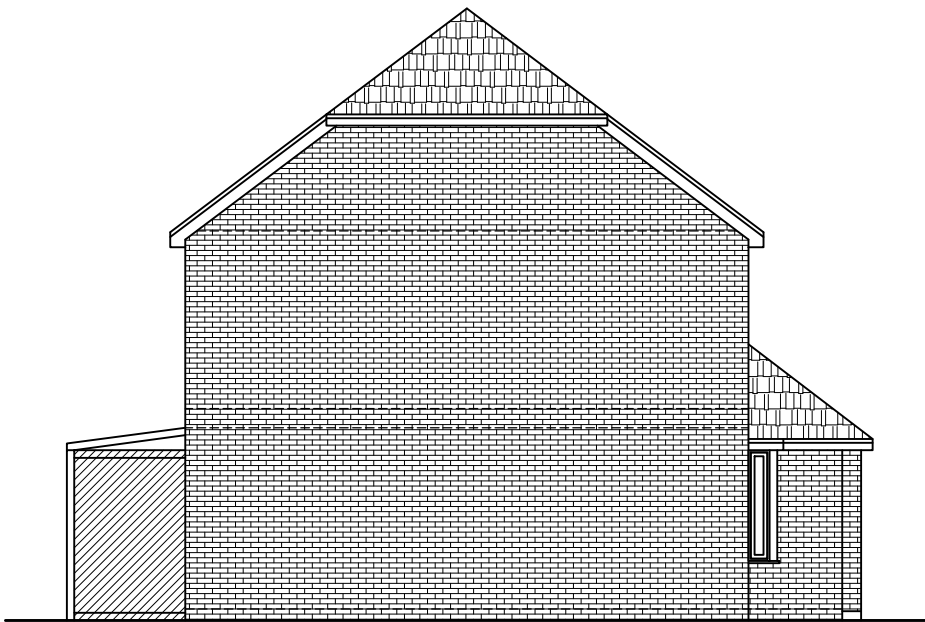
Existing Left Side Elevation Scale: 1/100
