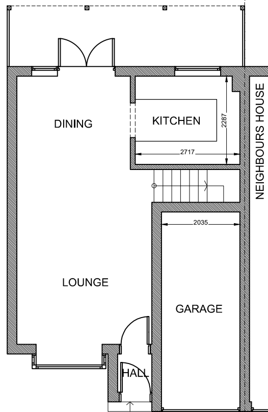
Pre-existing Ground Floor Plan Scale: 1/100
