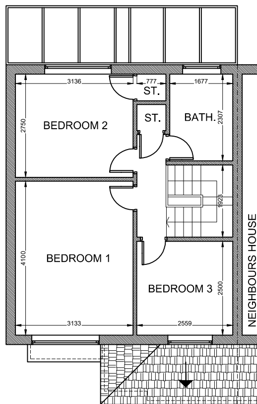
Pre-existing First Floor Plan Scale: 1/100
