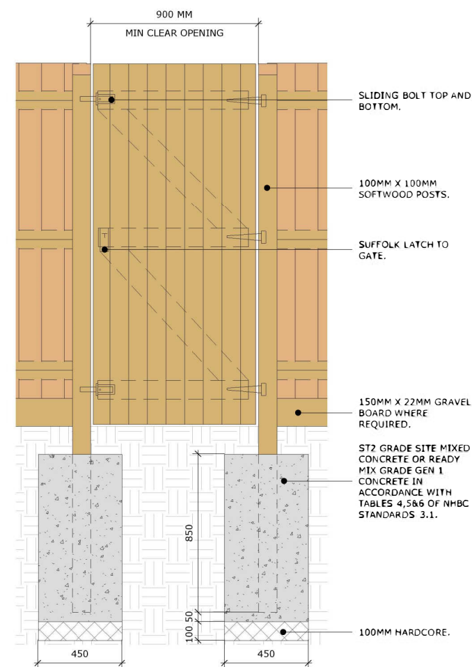
GATE ELEVATION
