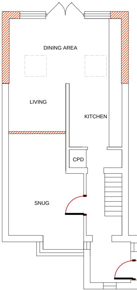
PROPOSED GROUND FLOOR PLAN scale 1-100
