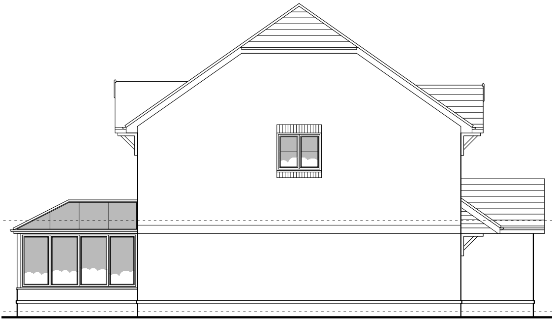
SIDE ELEVATION 1:100
