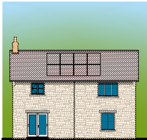
REAR ELEVATION
