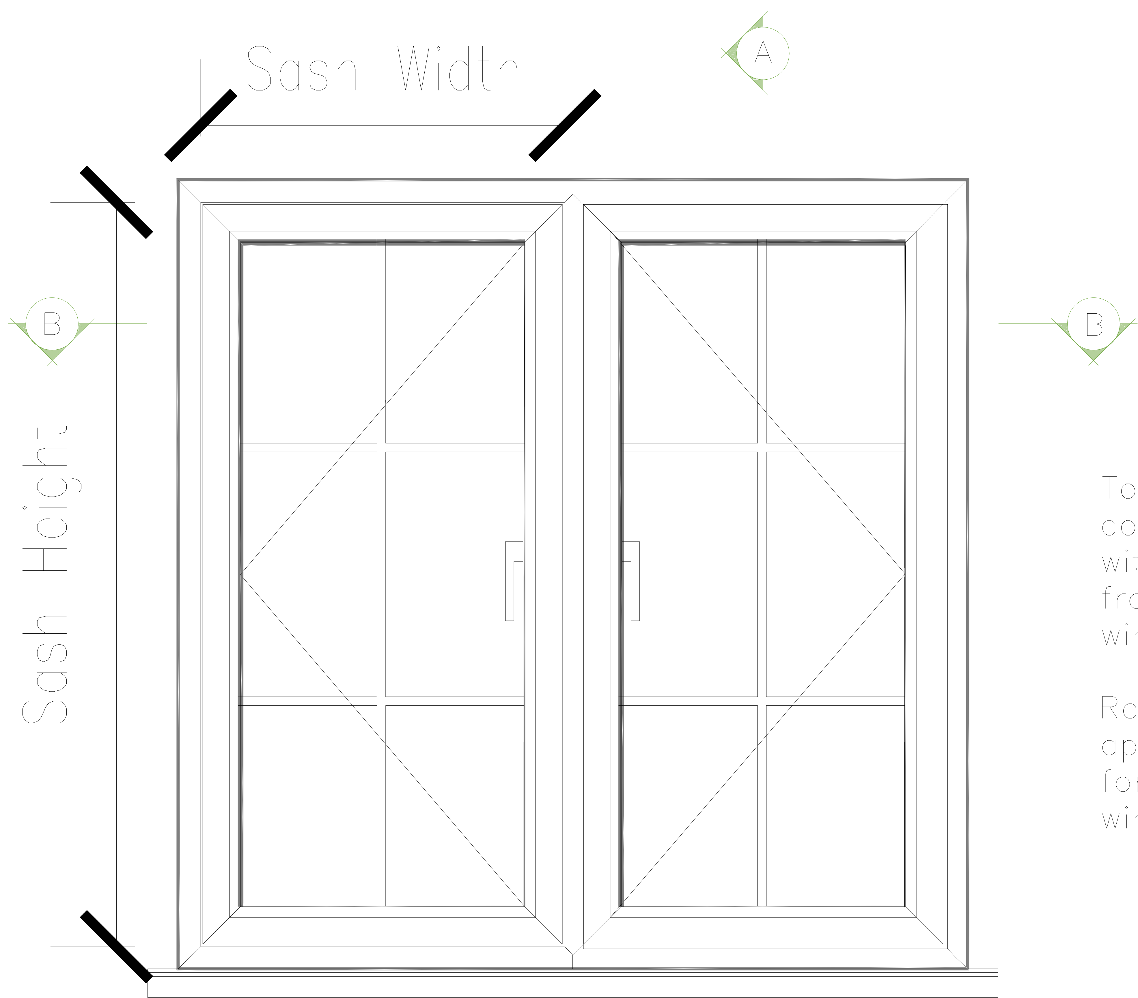
Typical Elevation — Double Viewed from outside Scale 1:5
