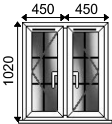
1 - 900w x 1020h (Basic Frame Size) 1 - 900w x 1050h, 30mm Cill Viewed Outside
