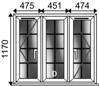
1 - 1400w x 1170h (Basic Frame Size) 1 - 1400w x 1200h, 30mm Cill Viewed Outside
