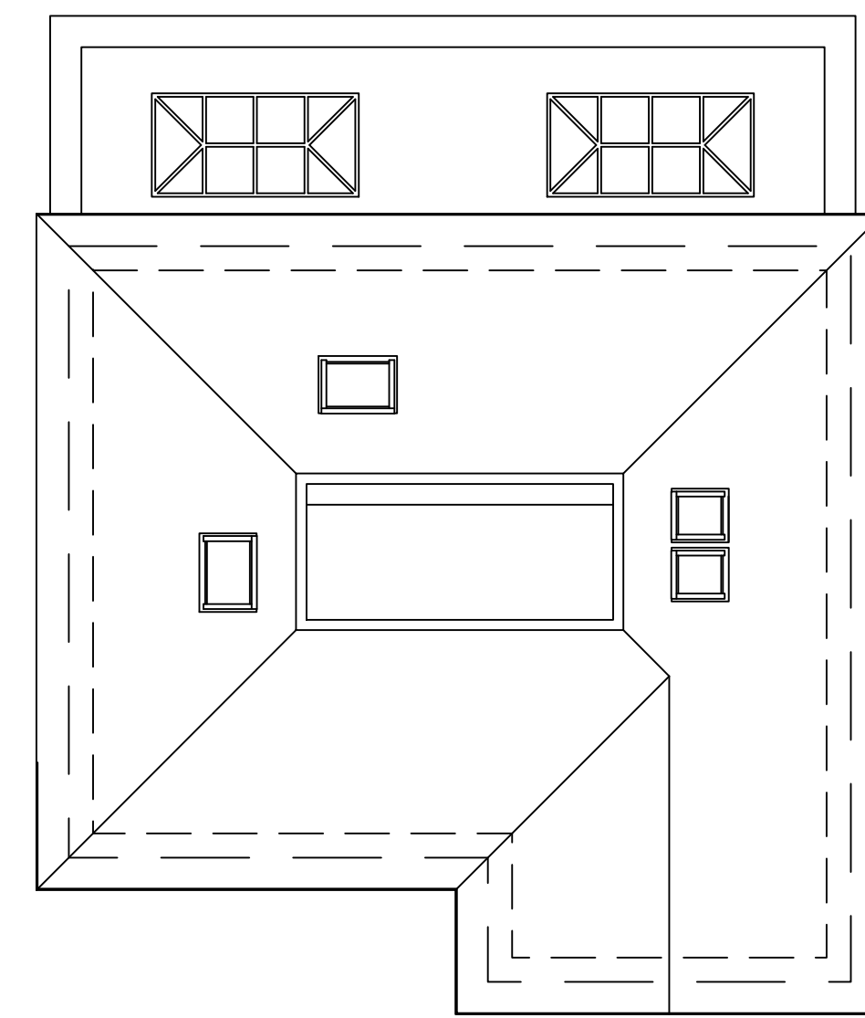
ROOF PLAN
