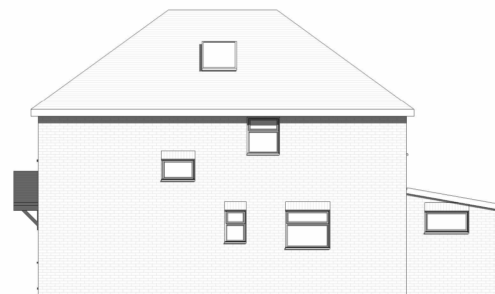
⑥ Existing Side Elevation_1 1 : 100
