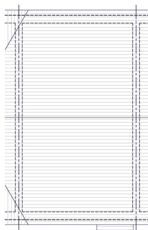
ROOF PLAN
