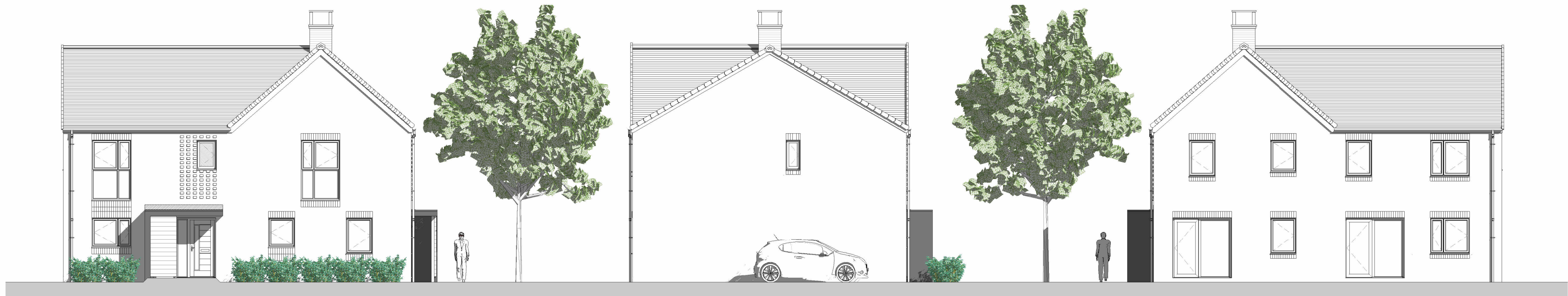
Front Elevation 1 : 100
