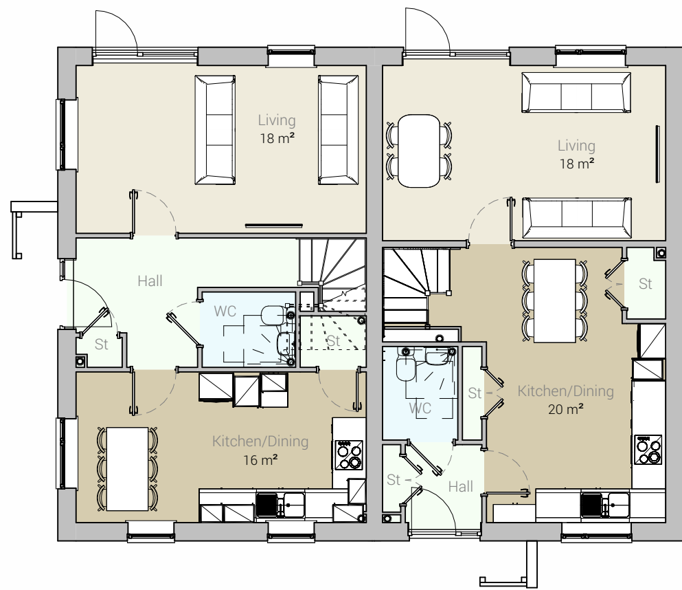
Ground Floor 1 : 100
