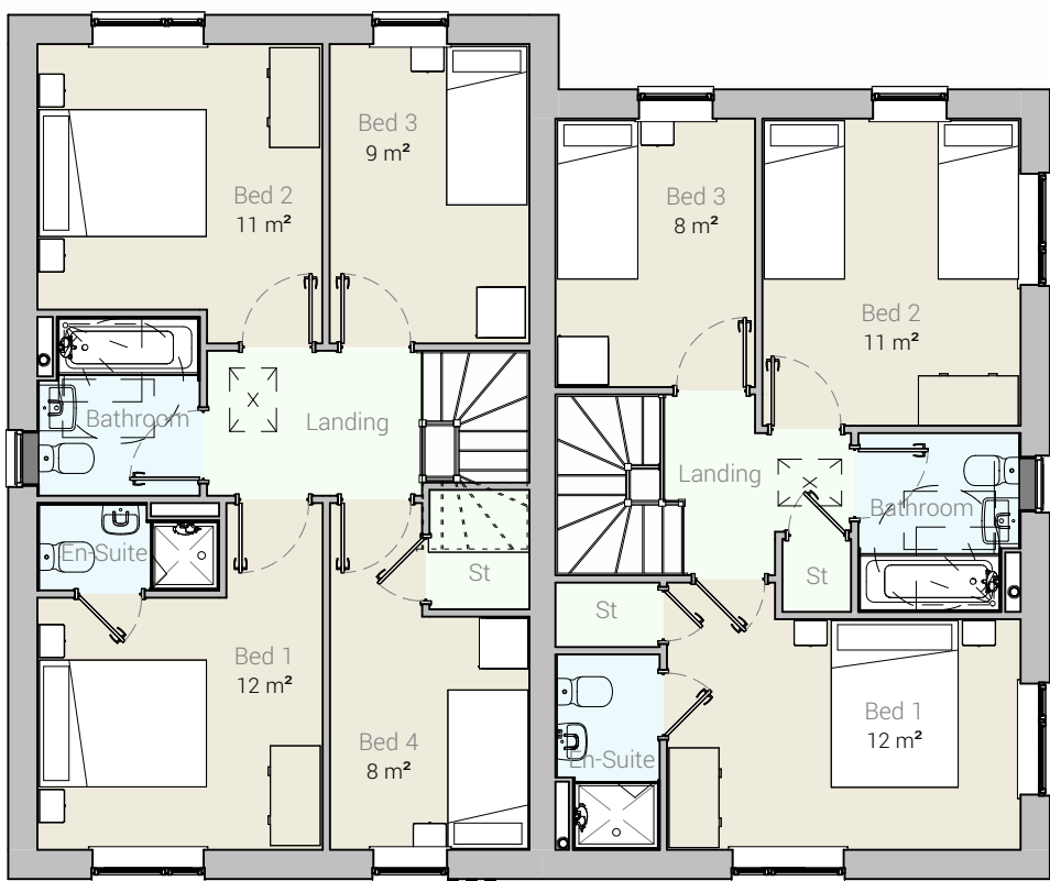
First Floor 1 : 100
