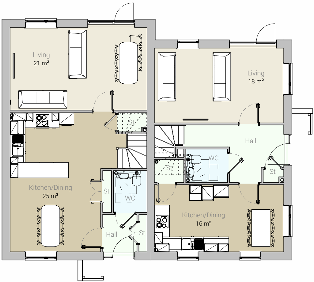
Ground Floor 1 : 100
