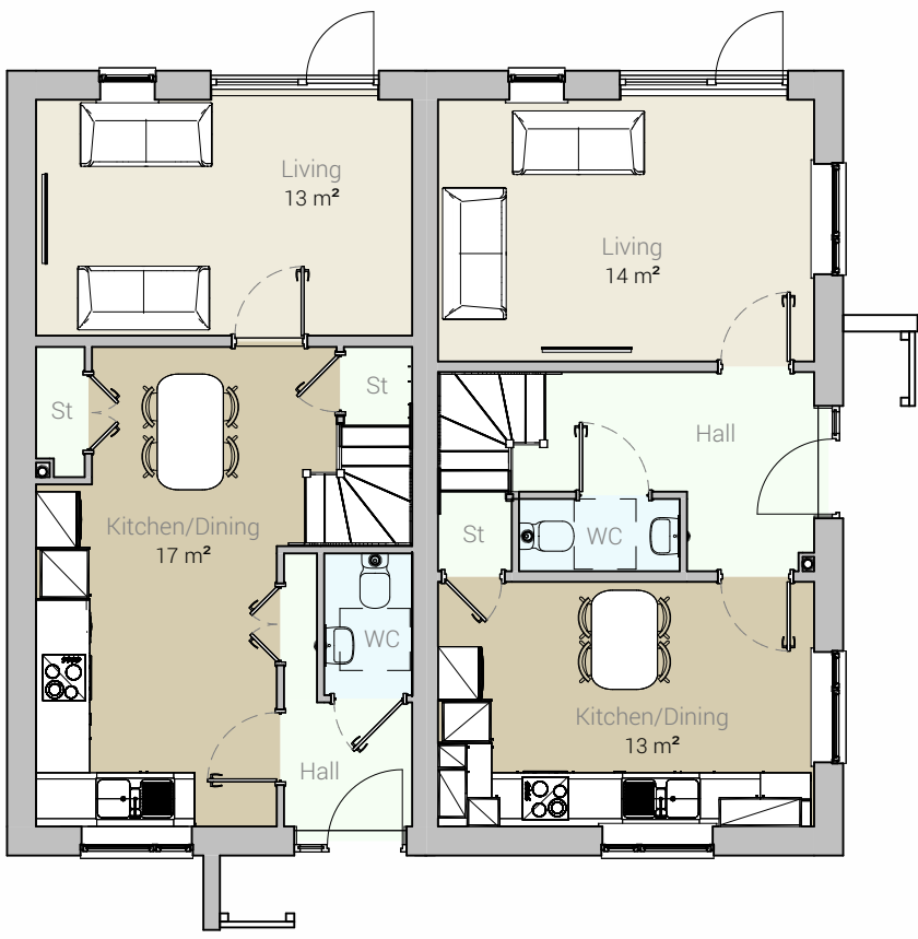
Ground Floor 1 : 100
