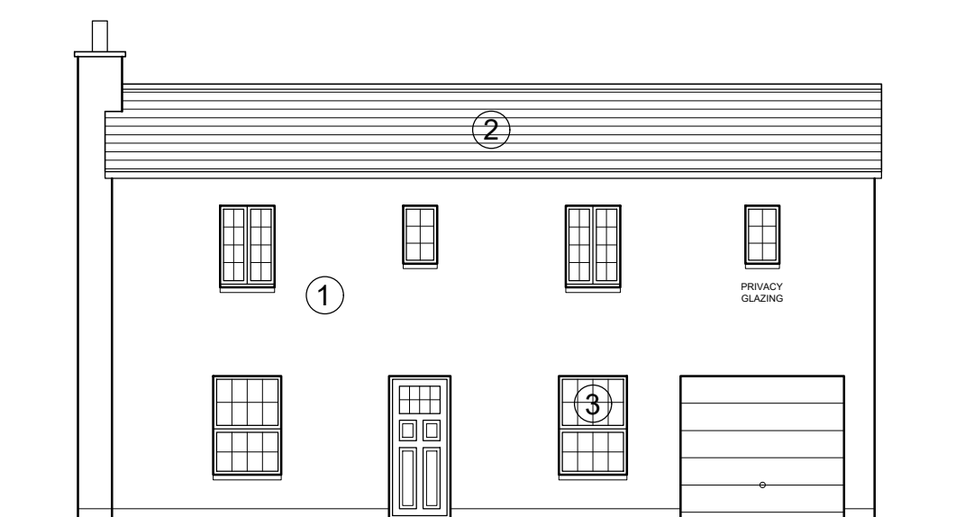
FRONT (EAST)
