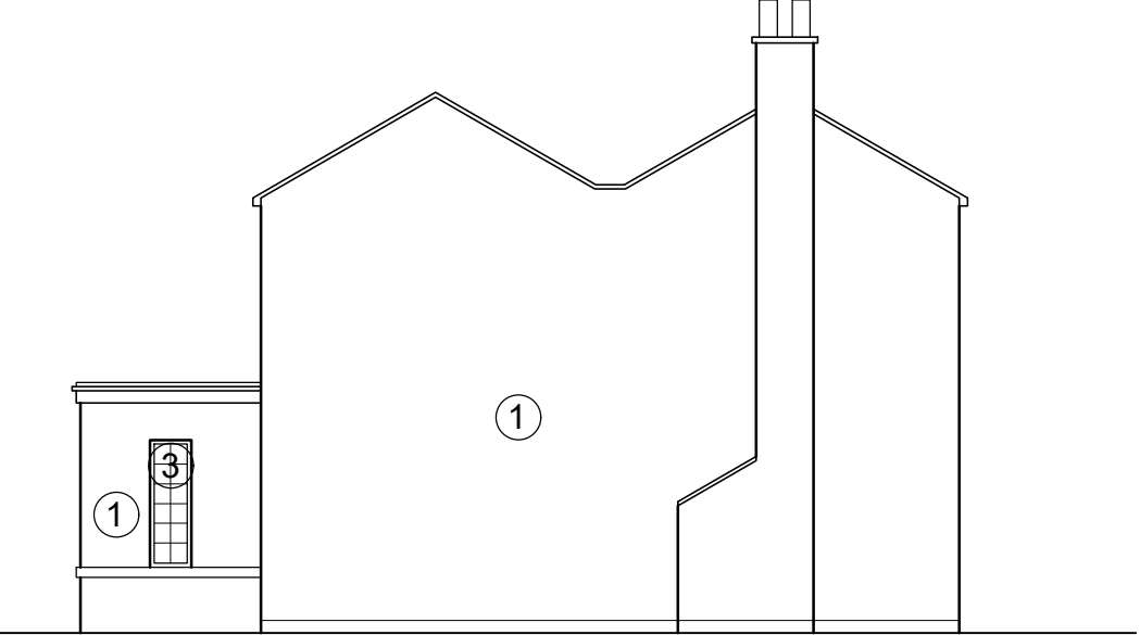
SIDE (SOUTH)
